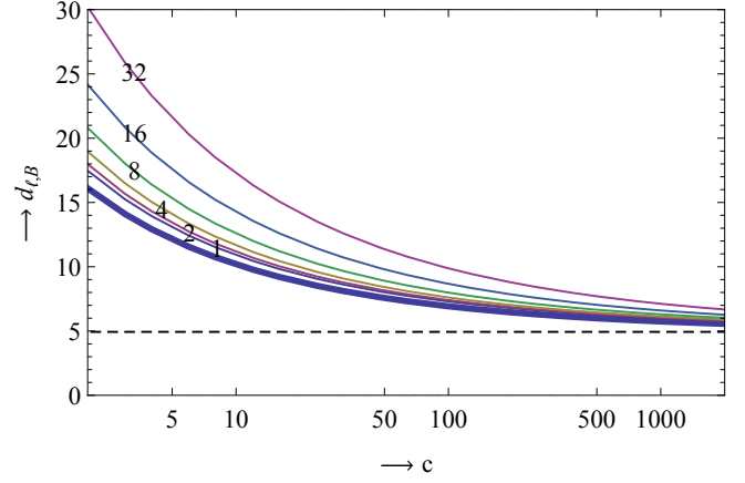
Fig. 4. Optimal values of d_{\ell,B} in the weakly dynamic Tardos scheme from Section IV-B, for the parameters n = 10^6 , \varepsilon_1 = \varepsilon_2 = 10^{-3} , and \eta = \frac{1}{3} . The bold curve corresponds to the values of d_\ell in the static Tardos scheme with the same parameters, while the six curves above this curve correspond to the optimal values of d_{\ell,B} for B = 1, 2, 4, 8, 16, 32 respectively. The dotted line corresponds to the asymptotic optimal value d_\ell = \frac{\pi^2}{2} \approx 4.93 . For B = 1 we get exactly the codeword lengths of the dynamic Tardos scheme.
