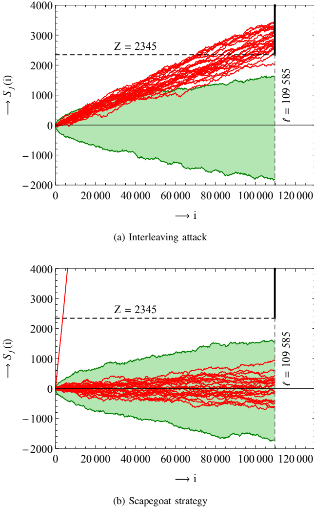
Fig. 1. Simulations of the Tardos scheme, with c = c_0 = 25 colluders, n = 10^6 users, and error probabilities \varepsilon_1 = \varepsilon_2 = 10^{-3} . The green, shaded area corresponds to the range of innocent user scores, the red lines correspond to pirate scores, and the dashed lines correspond to the threshold Z and codeword length \ell . In Fig. 1a the pirates used the interleaving attack (i.e. for each position, they choose a random pirate and output his symbol), and in Fig. 1b they used the scapegoat strategy. In both cases, the total coalition score S(\ell) at time \ell is approximately 72 000, but while in the first case the score is evenly divided among the pirates, in the second case one pirate takes all the blame.
